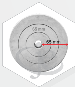
CB45 ROUND 65 mm 04 CAVITY ID : 20 Thickness : 35 mm
